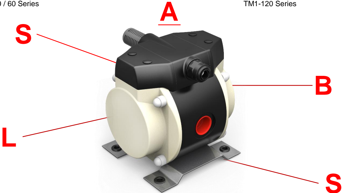
KF103-003 High Speed POM-C/ALU Air Motor kit for TM1-30 / 60 Series
